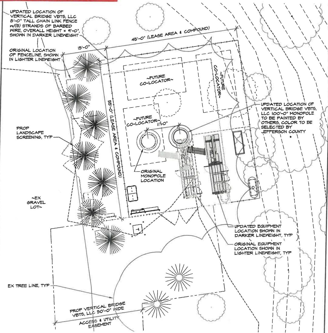
MONOPOLE & COMPOUND OVERLAY SCALE: 1" = 15'
